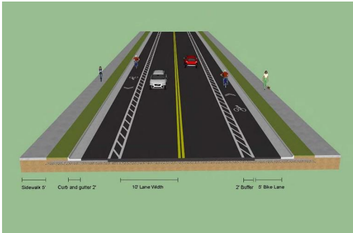
Typical Section
