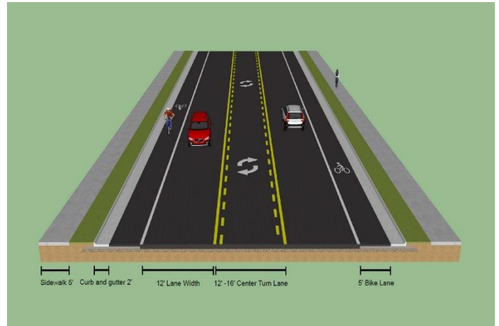
Typical Section with Turn Lanes
