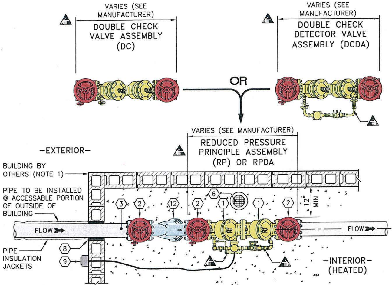
PLAN VIEW
